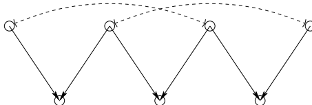
Fig. 1. A constraint graph with no solution.
