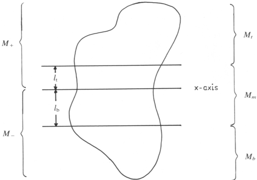
Figure 1. Cuts in M .
