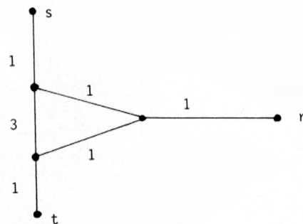
Fig. 1. S = \{r, s, t\} , d_1(s, t) = 4 , but d'_1(s, t) = 5 .
