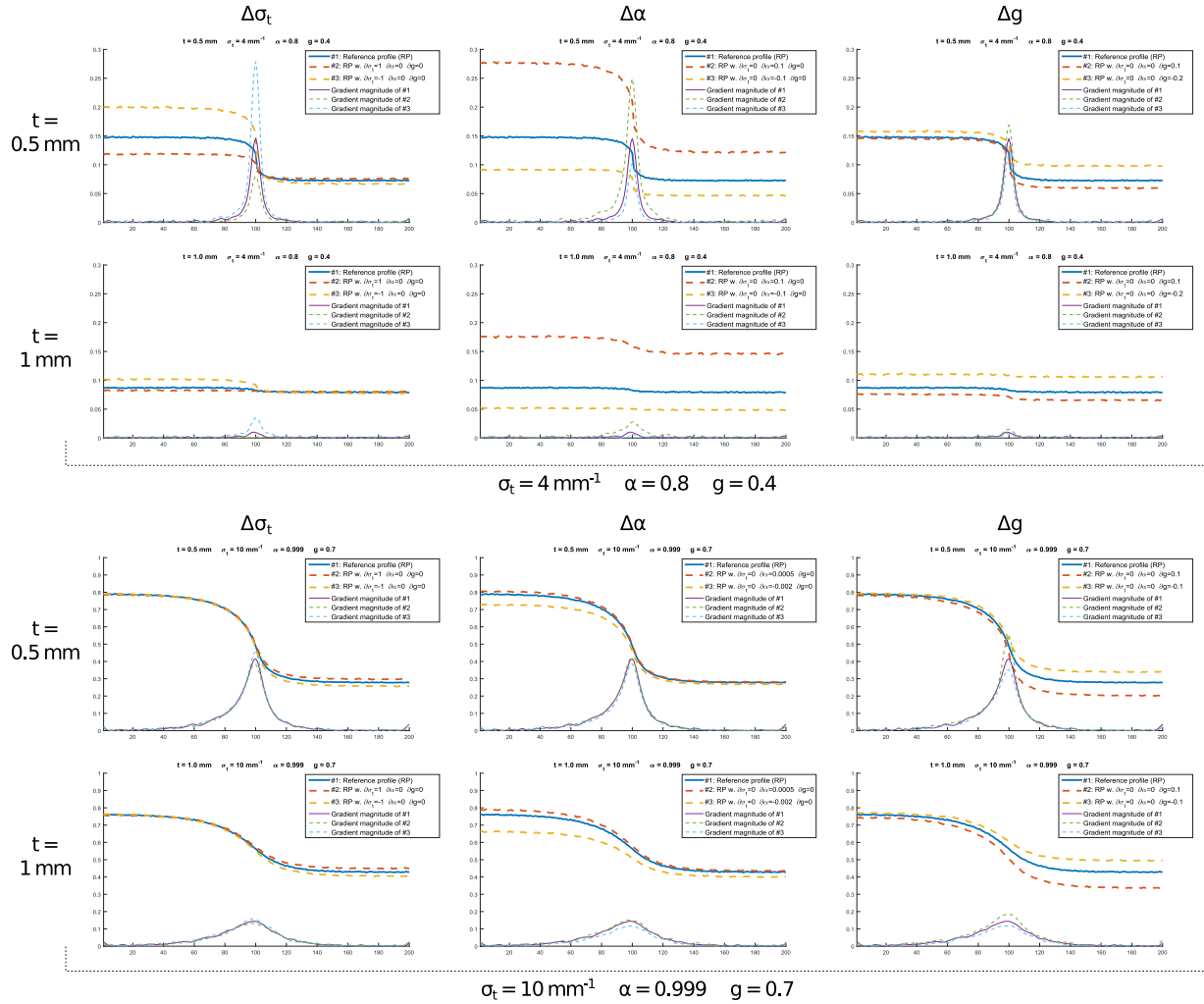
Fig. 3. Edge profiles simulated with our virtual setup (Sec. 4.3) for two different parameter sets \in \mathcal{V} , each for two sample thicknesses t \in \{0.5, 1\} \text{ mm} . Starting from a reference profile (solid blue), each plot shows two profiles resulting from a small change along one of the three dimensions of \mathcal{V} (dashed red and yellow). We also compare the respective profile gradient magnitudes, since these are taken into account by our fitting (Sec. 5.5). Details are listed in the corresponding plot legends. Please also note the different ranges in the two plot sets.
