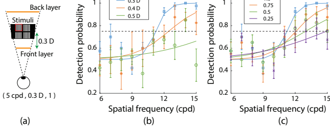
Fig. 3: The configuration of displays and stimuli (a). The probability of detecting the difference between LB and LFS methods for various depth (b) and contrast levels (c).
