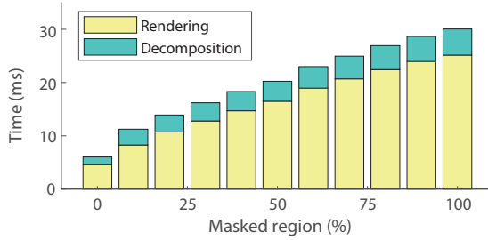
Fig. 11: The rendering and decomposition timings for various ratios of masked region for the fish scene in Fig. 12.
