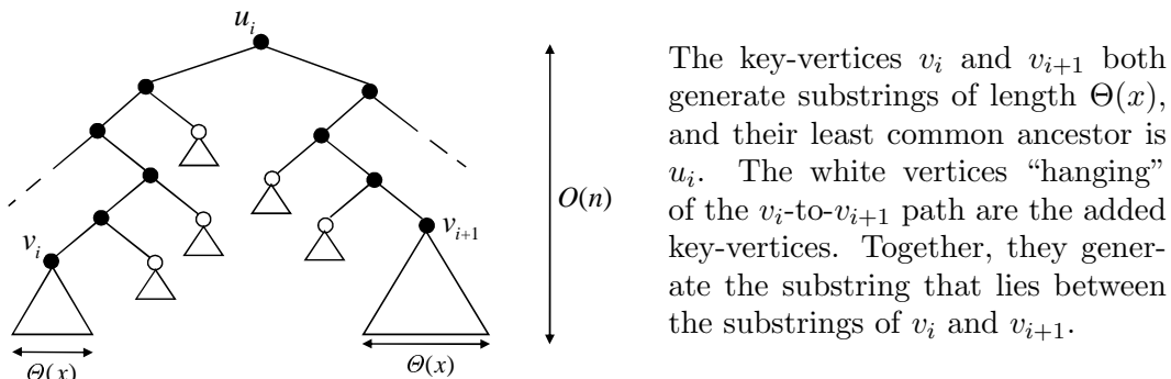
Figure 3: A closer look on the parse tree of an SLP \mathcal{A} .
