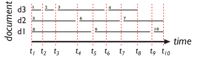
Figure 2: Sublist Materialization
