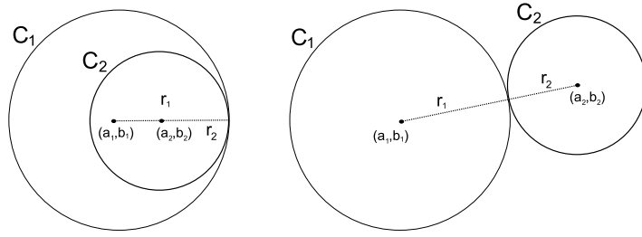
Figure 2: Given two circles C_i , i = 1, 2 , with midpoints (a_i, b_i) and radii r_i = \sqrt{c_i} , there are two degenerate situations of tangential intersection.
