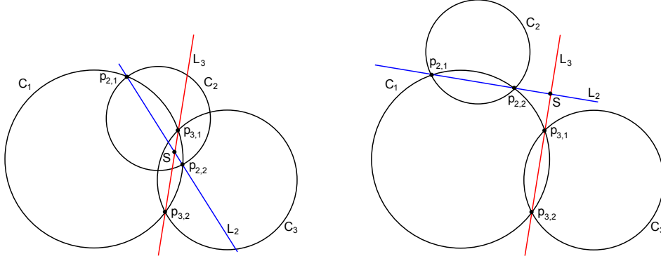
Figure 3: The location of the intersection point S = L_2 \cap L_3 with respect to C_1 determines whether the two pairs of points \{p_{i,1}, p_{i,2}\} , i = 2, 3 are interleaving or not.
