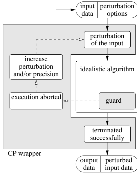
Figure 4: The control flow of the general CP template.
