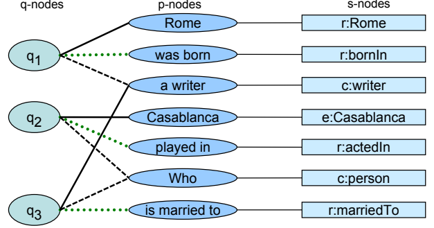
Figure 4: Computed subgraph for the running example.
