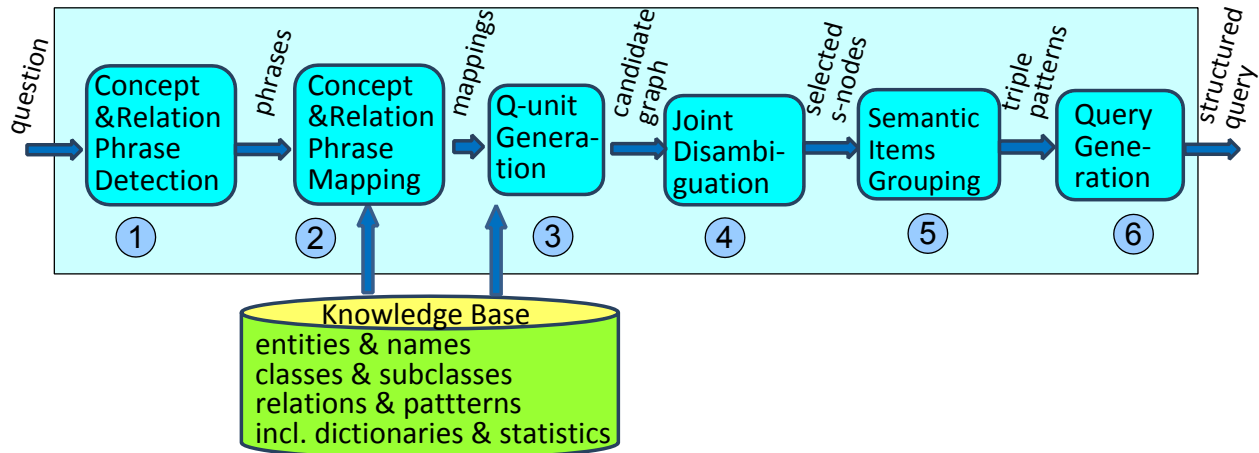
Figure 2: Architecture of DEANNA.
