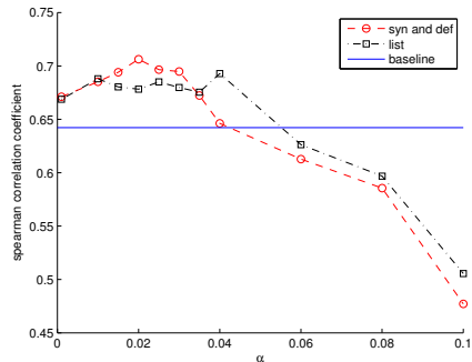
Fig. 2. Spearman’s \rho on the wordsim-353 dataset
