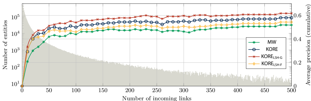
Figure 3: Accuracy of relatedness measures on entities with fewer than 500 incoming links on the KORE50 dataset
